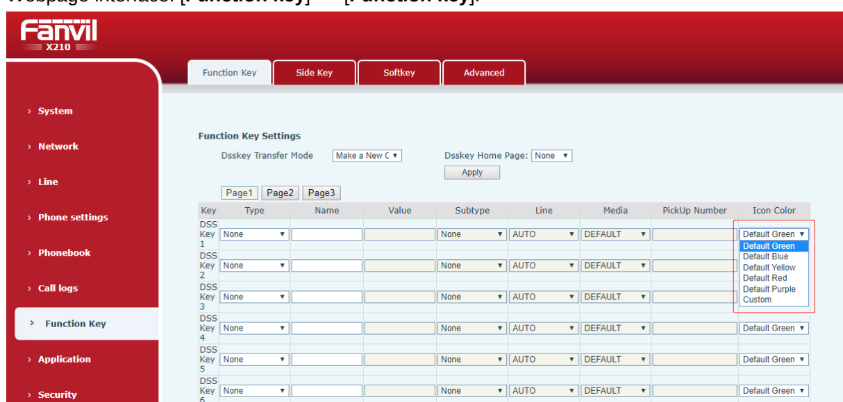
Picture 107 - DSS settings
